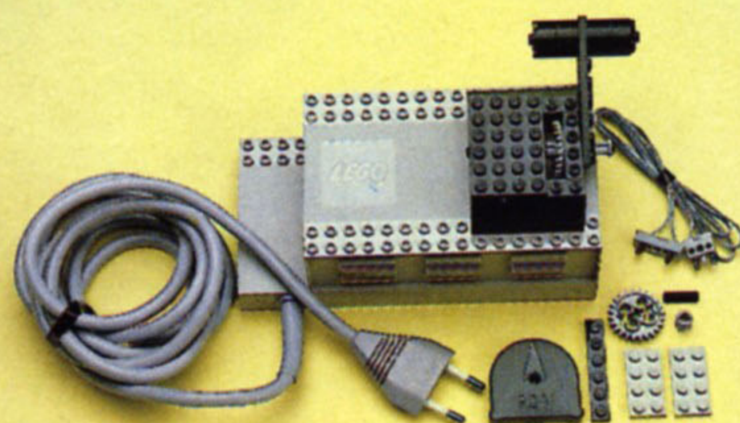
7864 12 Volt transformer/controller. Around £35.00
